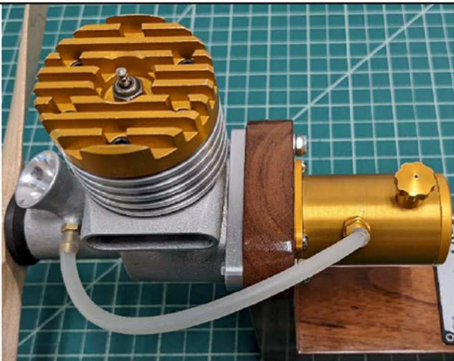
Titan .60 Glow-plug Engine Designed by George Genevra Built by Mark Presling
